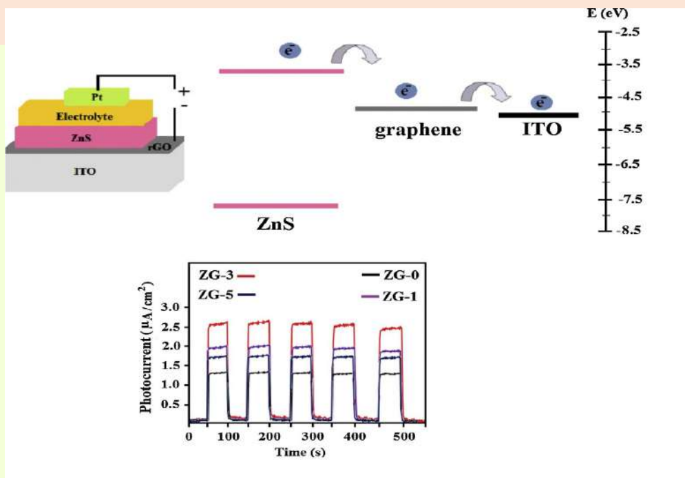
Photocurrent versus time (I-t) curves of the solar cell device based on pure ZnS and ZnS-rGO composite with different mass ratios of rGO (1, 3 and 5 wt%)
