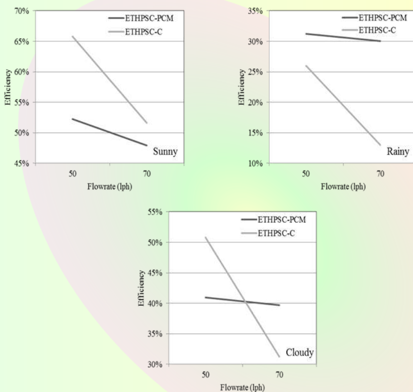
Comparison of efficiency in conventional model (ETHPSC-C) and new design (ETHPSC-PCM)
